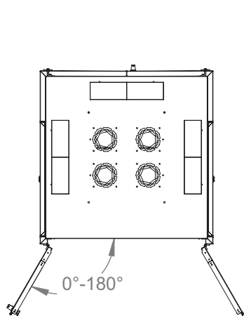
Front door opening view
