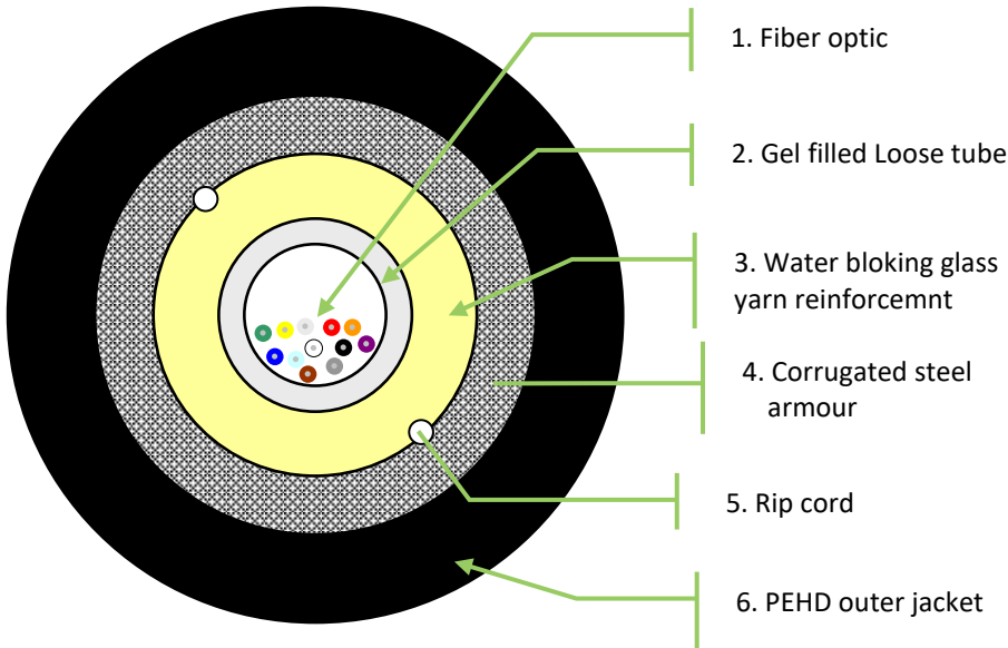
Drawing for information only (depends of fibers' number)
